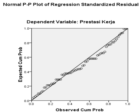
Gambar 1 Normal Probability Plot Hasil Pengujian Normalitas Data
